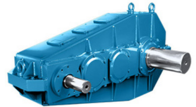
CRANE DUTY GEARBOX
